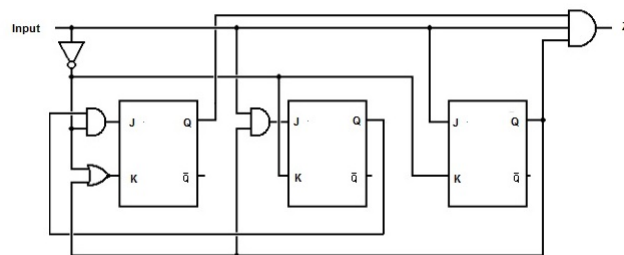
Fig. 7. Schematic of a Conventional 11011 sequence detector
