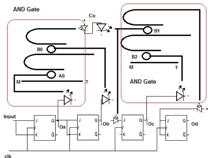
Fig. 6. Schematic of a 4 bit Optoelectronic Counter
